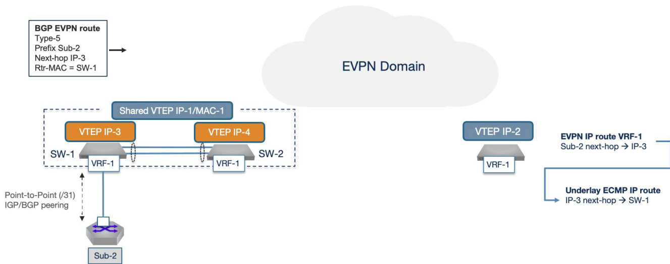
Figure 10: EVPN with MLAG, optimal forwarding for single-homed layer 3 nodes
