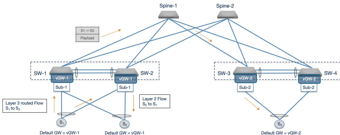
Figure 2: MLAG optimal layer 2 and 3 forwarding under steady-state conditions
