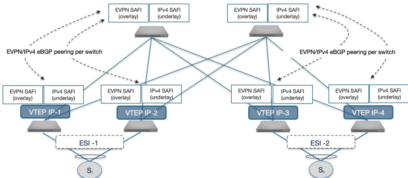
Figure 16: BGP EVPN/IPv4 peering sessions with an EVPN A-A topology
