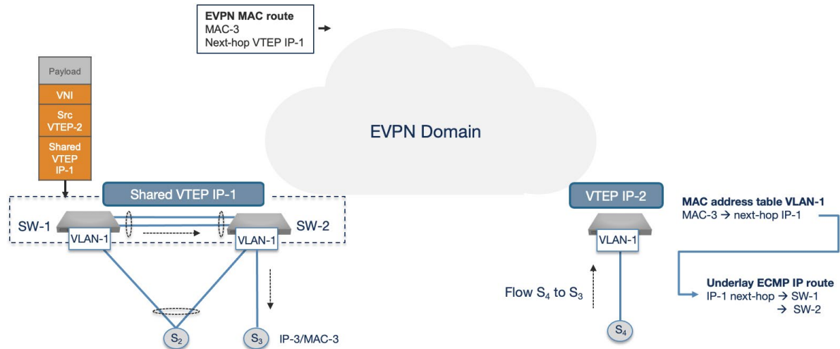
Figure 7: EVPN with MLAG, forwarding model for single-homed nodes
